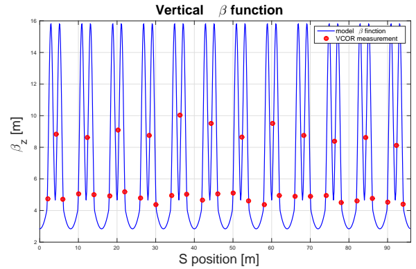
Figure 5: Vertical \beta function measured in HCM and VCM corrector magnets locations.
