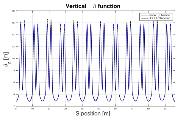
Figure 7: Vertical \beta function obtained using LOCO algorithms.
