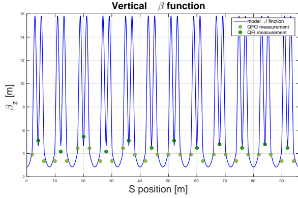
Figure 3: Vertical \beta function measured in SQFO and SQFI magnets locations.
