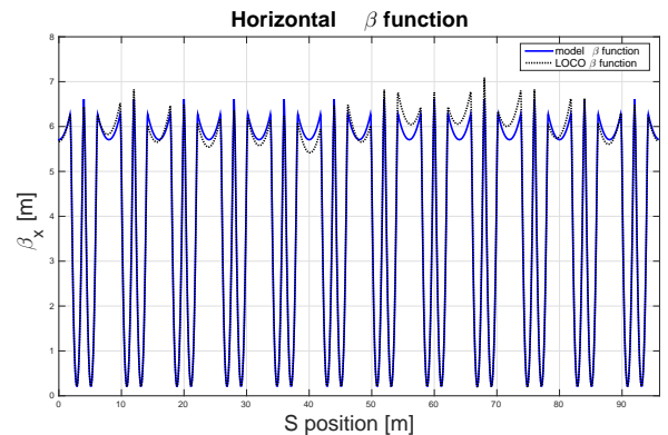
Figure 6: Horizontal \beta function obtained using LOCO algorithms.
