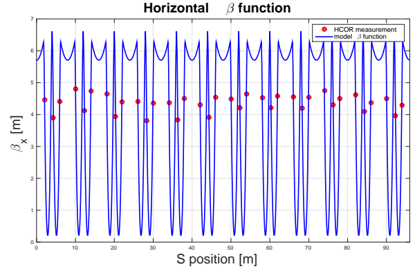
Figure 4: Horizontal \beta function measured in HCM and VCM corrector magnets locations.
