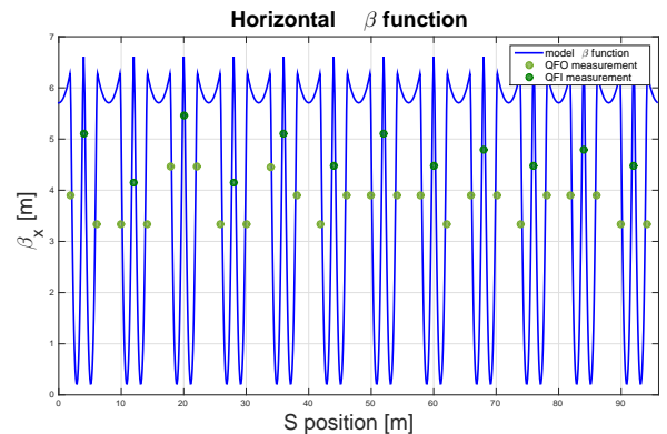
Figure 2: Horizontal \beta function measured in SQFO and SQFI magnets locations.
