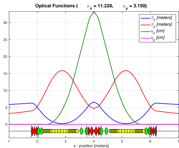
Figure 1: Twiss functions in DBA cell.
